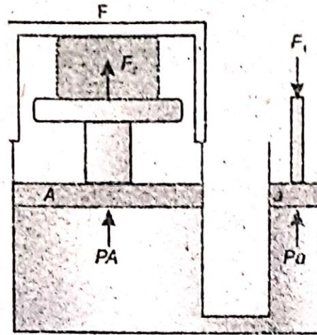
Fig. A hydraulic press.
